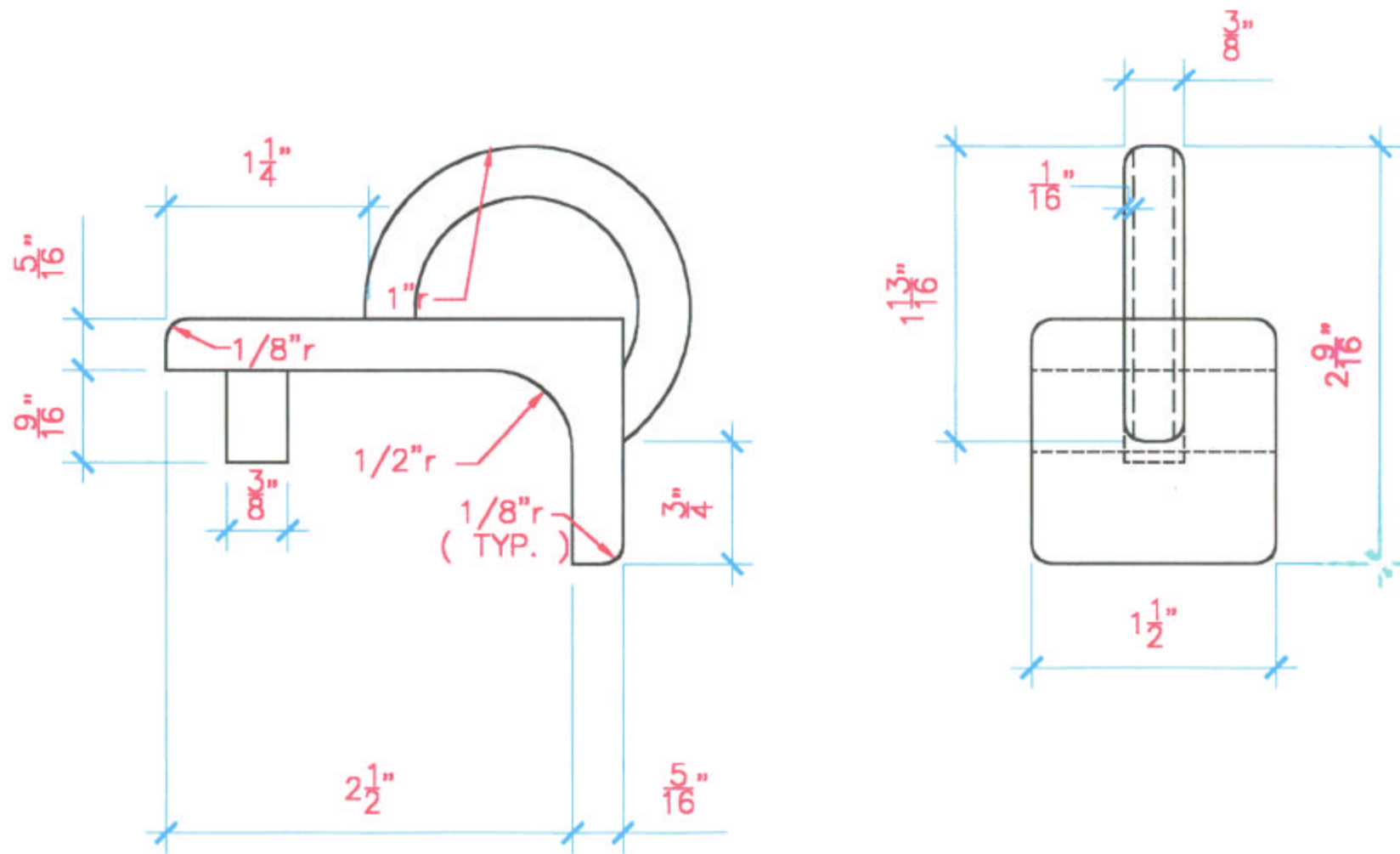
2.0" Solid Disk - Radius Corner "20SDR"
