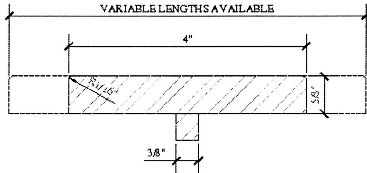
SIDE WALL "SW"
