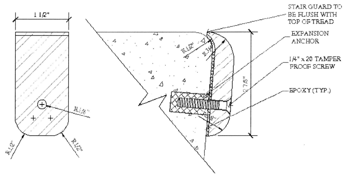
STAIR GUARD 0.5" RADIUS CORNER "SG.5R"
